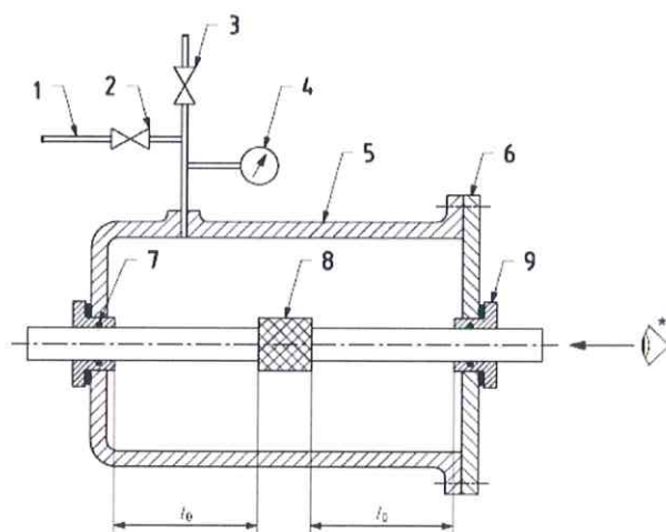
Figure 1 — Typical apparatus
