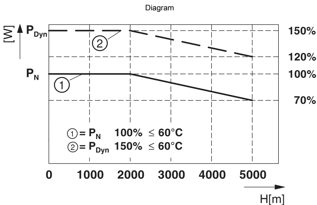
Altitude-dependent derating
