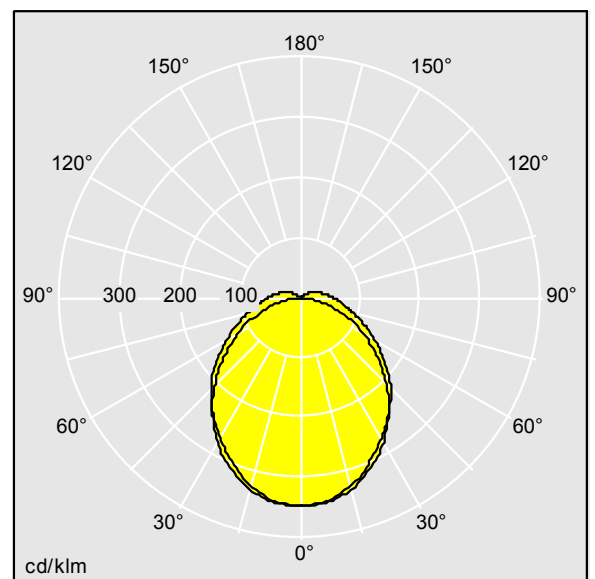
D42271AA_AQFPRO_S_LED5200-840_PC_MB_HF.ltd
