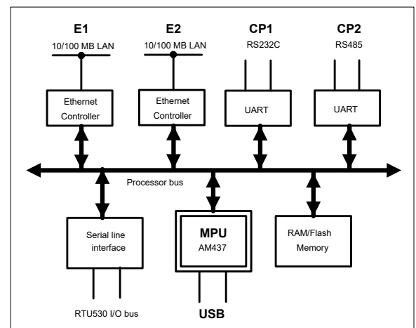
Figure 1: Block diagram communication unit
