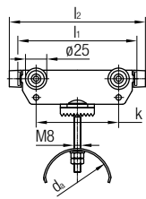
Cable Trolley
