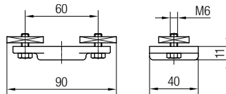
End Clamp
