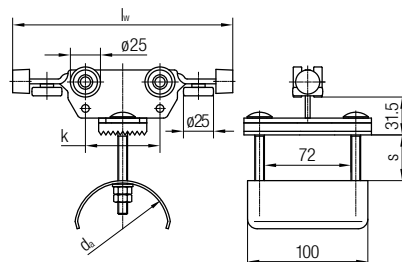
Cable Trolley
