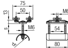
End Clamp
