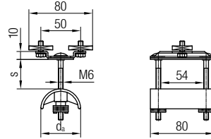
End Clamp
