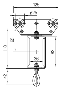
Towing Trolley
