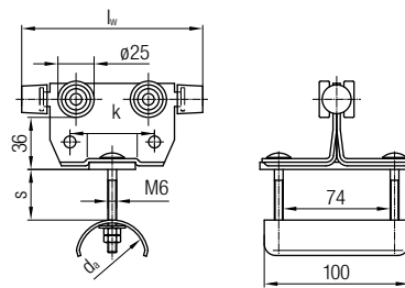
Cable Trolley
