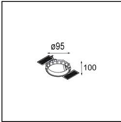
12500230 Recessed ring 82
