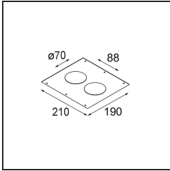
12291030 Gypkit 210x190-2xØ70
