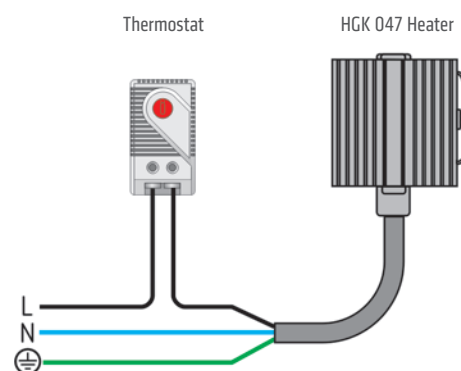
Wiring example
