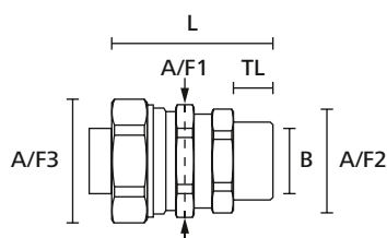
HelaGuard compression fitting, straight with swivel external thread
