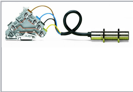
Sensor terminal block paired with a 3-conductor sensor (ground connection)
