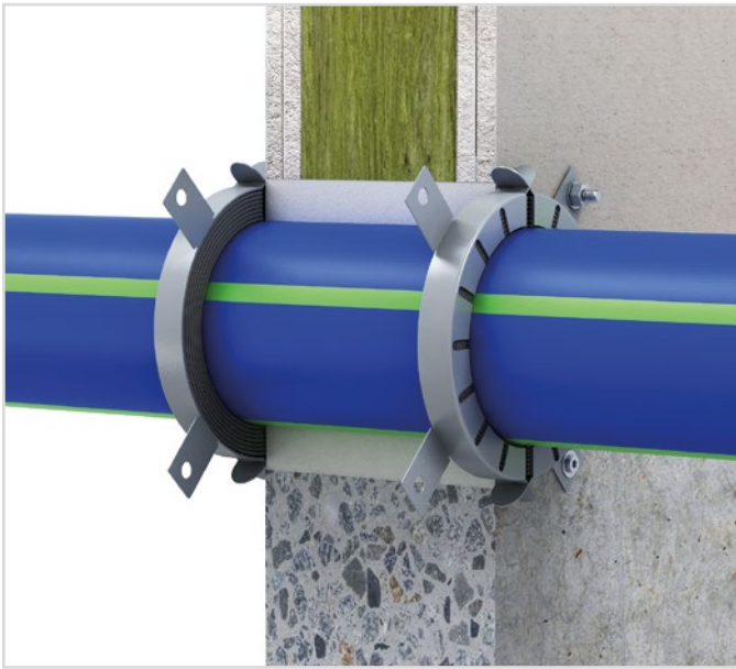
Application of the fire protection sleeve AWM II in the wall
