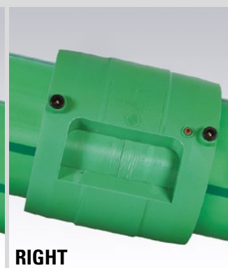
Push the second pipe – also peeled and cleaned – into the socket
