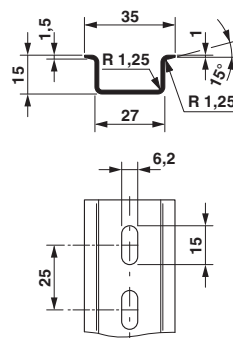
Dimensioned drawing
