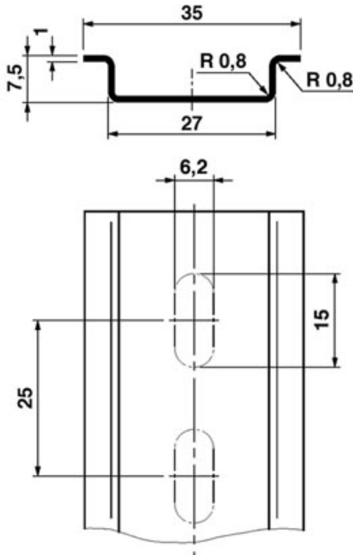
Dimensioned drawing
