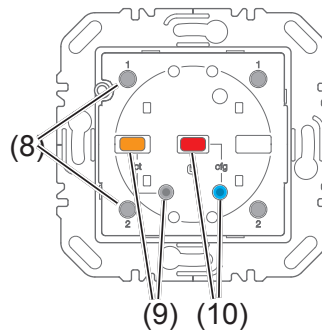
Figure 2a: Operating elements of the 1gang radio button
