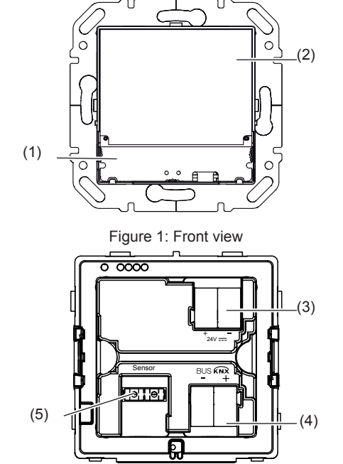
8044 01 00 KNX thermostat with display and integrated bus application unit
