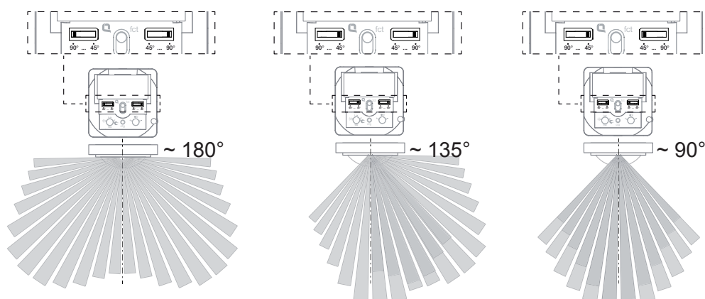
Fig. 7: Setting the detection angle
