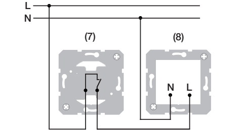
Figure 2: Connection example of LED signal light, white lighting
