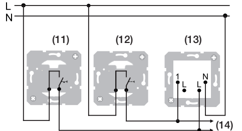
Figure 5: Connection example of colour switching via outer conductor, not looped
