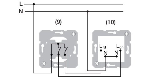
Figure 3: Connection example of LED signal light, red/green lighting
