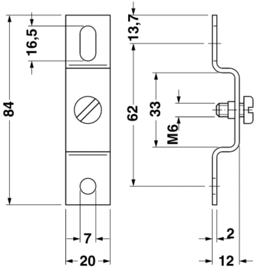
Dimensioned drawing
