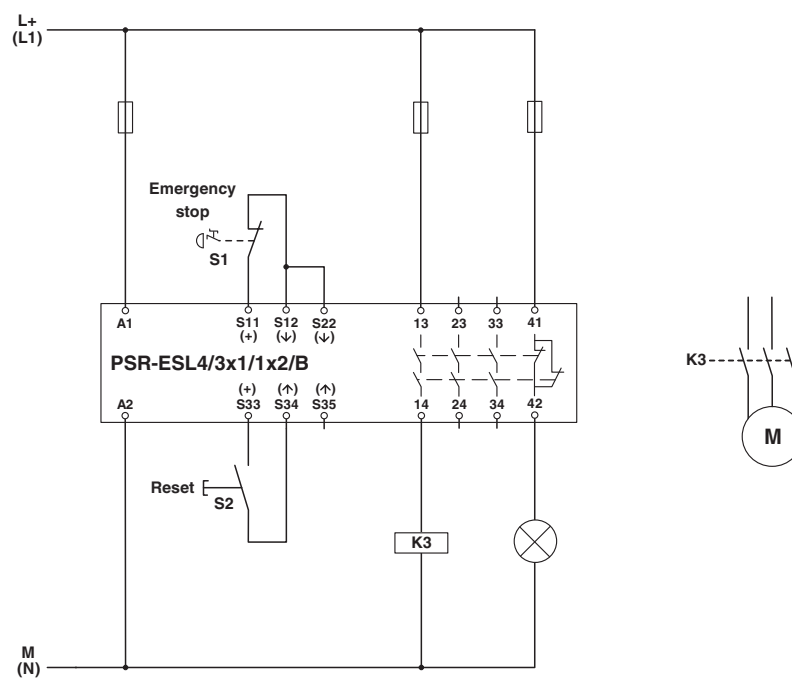
Circuit diagram
