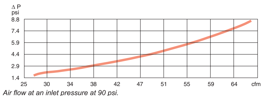
Flow chart. ErgoQIC 08 M15U and ErgoNIP 08 M10U
