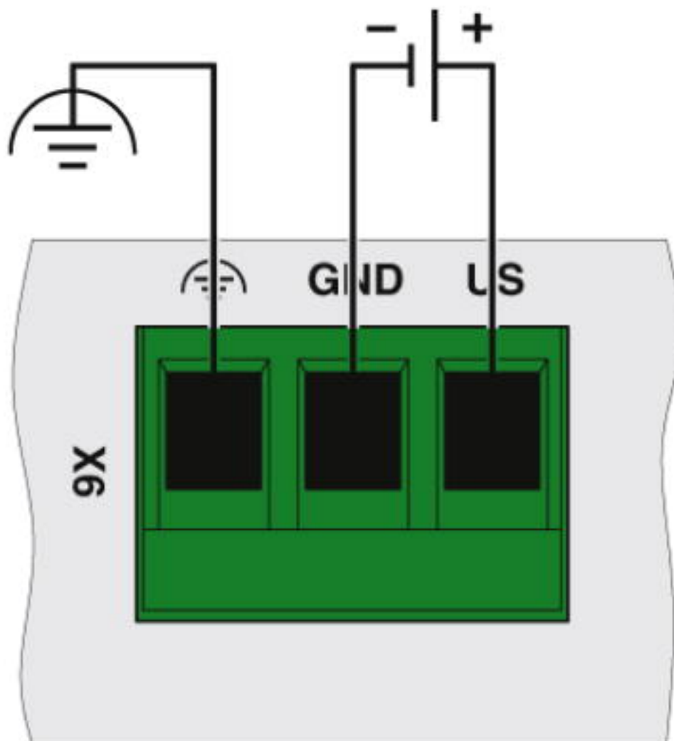
Connection diagram
