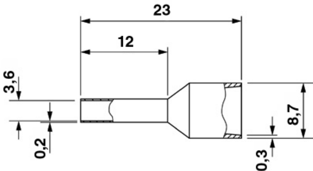
Dimensioned drawing
