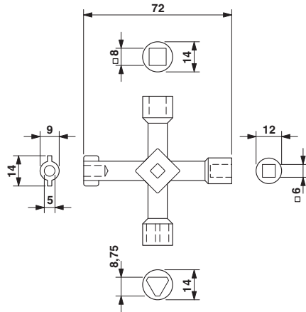
Dimensioned drawing
